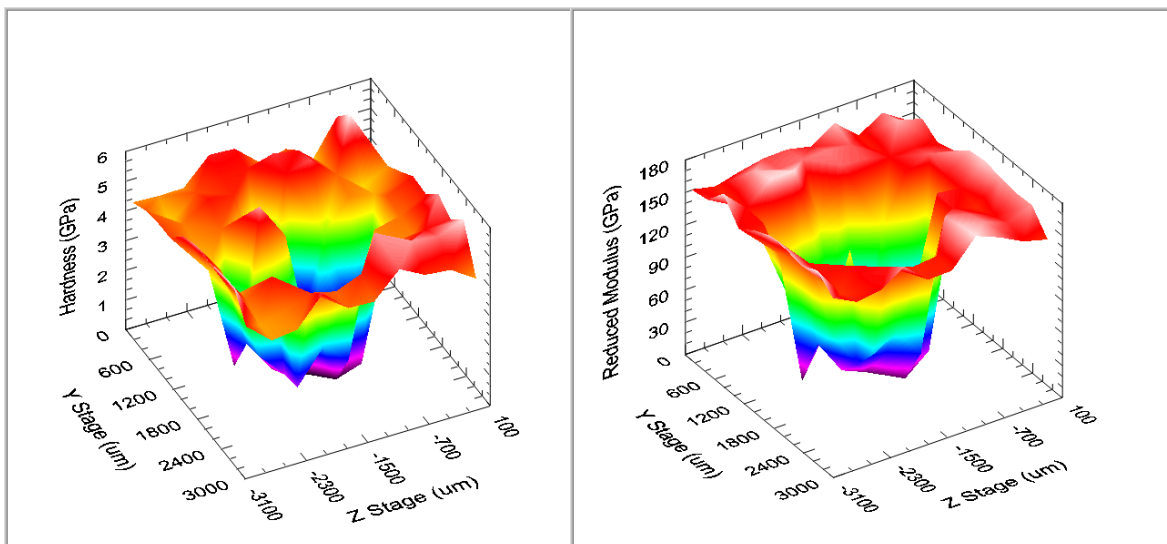
Fig. 5. Hardness and elastic modulus maps for titanium alloy (Ti6Al4V); Test conditions: \pm 100\mu\text{m} displacement amplitude, 5HZ frequency, 80N normal load, 2000 fretting cycles.
