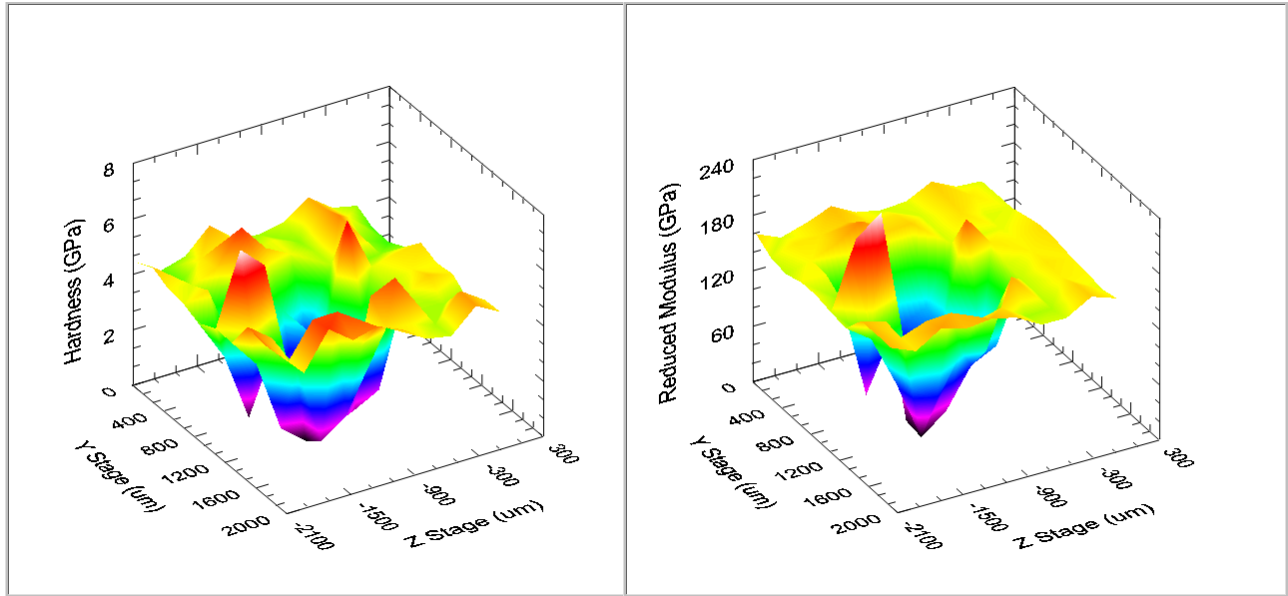
Fig. 4. Hardness and elastic modulus maps for titanium alloy (Ti6Al4V); Test conditions: \pm 100\mu\text{m} displacement amplitude, 5HZ frequency, 20N normal load, 10000 fretting cycles.
