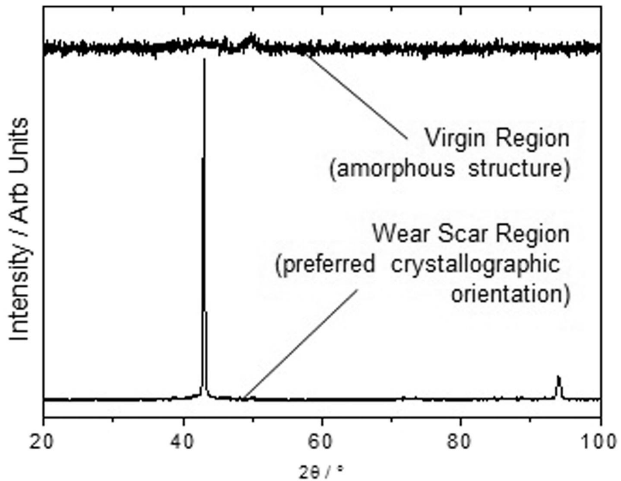
Fig. 9. XRD spectrum for copper; top line – virgin region of the sample; bottom line – worn surface.
